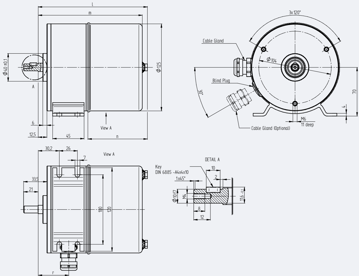
Steel sheet housing B3
